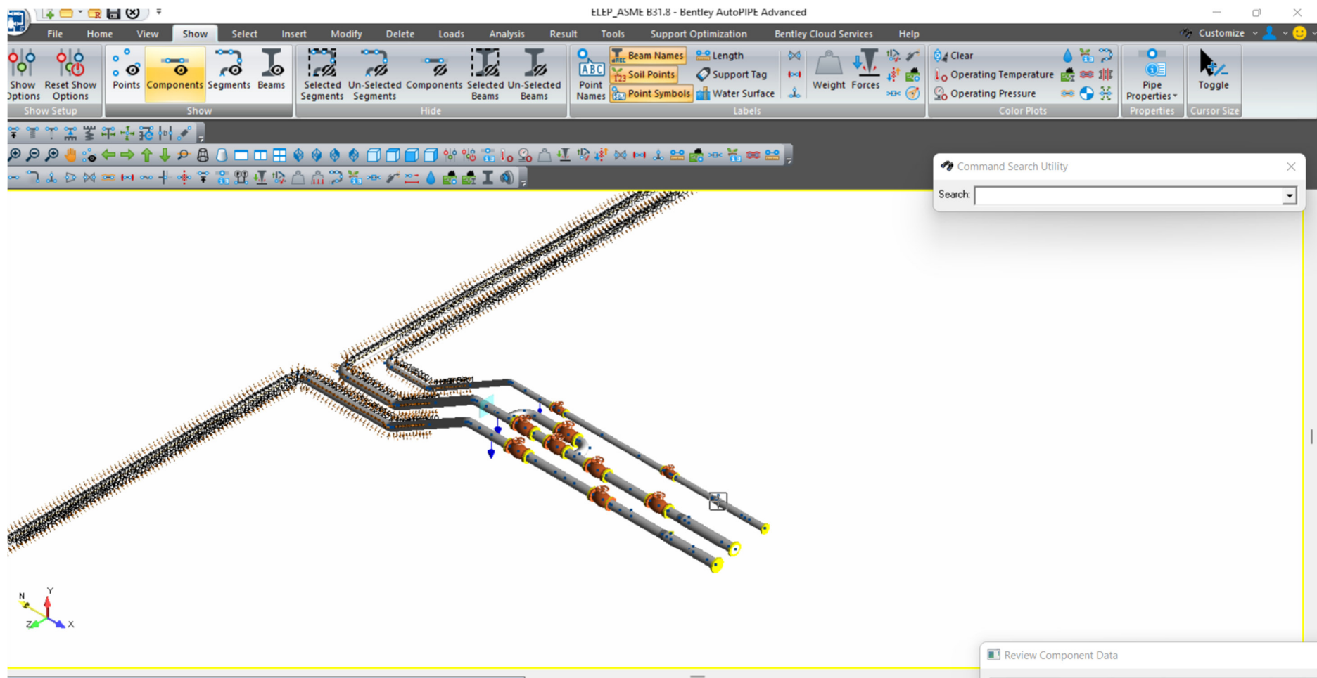
3 ASME B31.8 SCOPE (SUPPORT HIDDEN FOR CLARITY)
